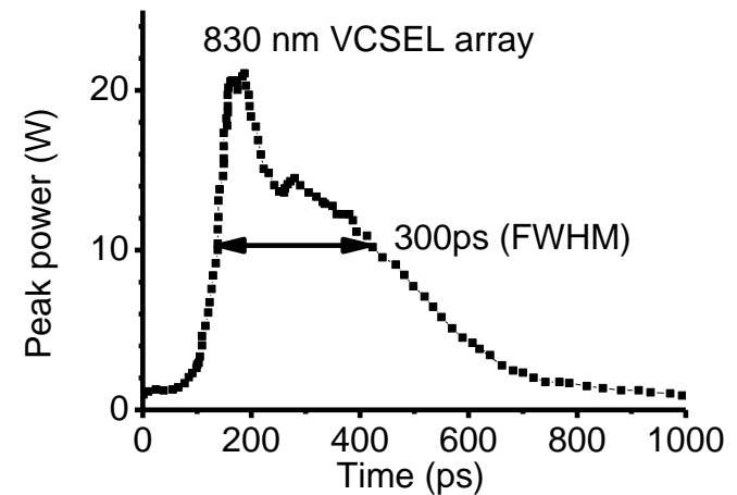
Optical pulse: 300ps pulse width (20W peak power)
