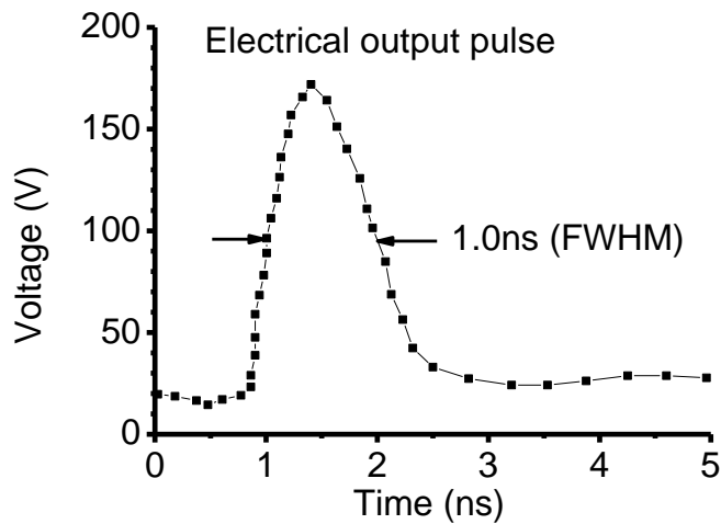
Electrical pulse: 1ns pulse width
